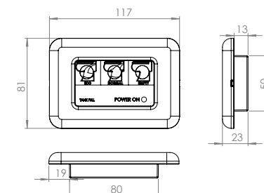
Electronic keyboard LUXE
