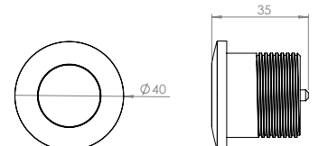
Push button COMFORT PLUS
