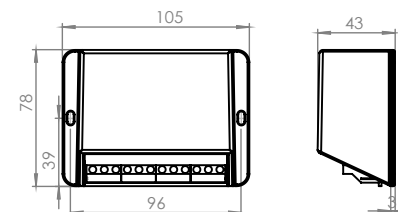
Electronic control box LUXE, COMFORT LUXE, COMFORT PLUS
