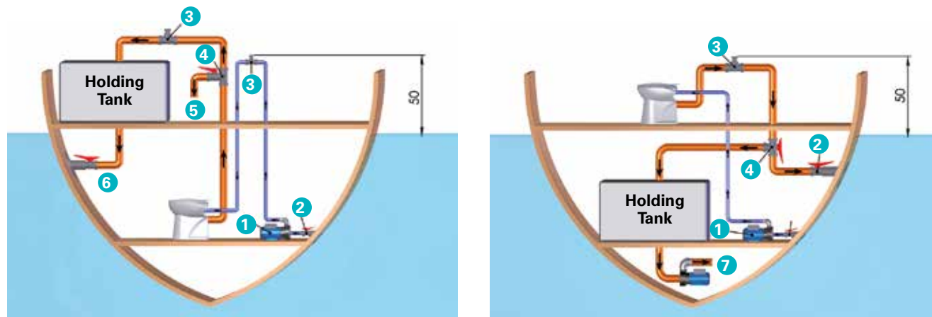
WC above sea level, holding tank below sea level
